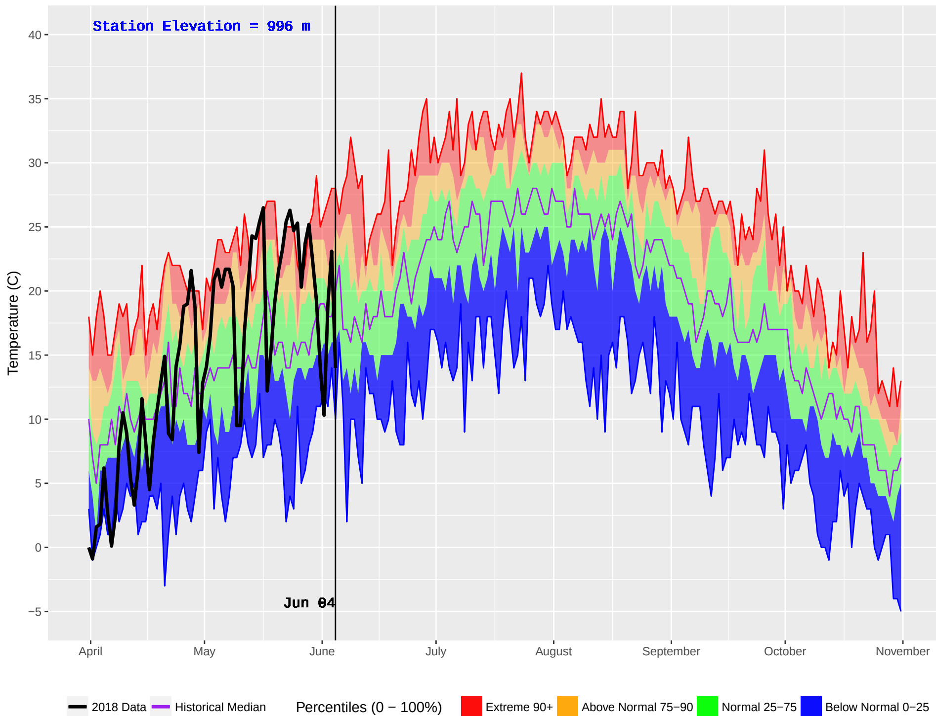
CRANBROOK FS (426) : Historical (2001–2016) and Current (2018) Noon Temperature
