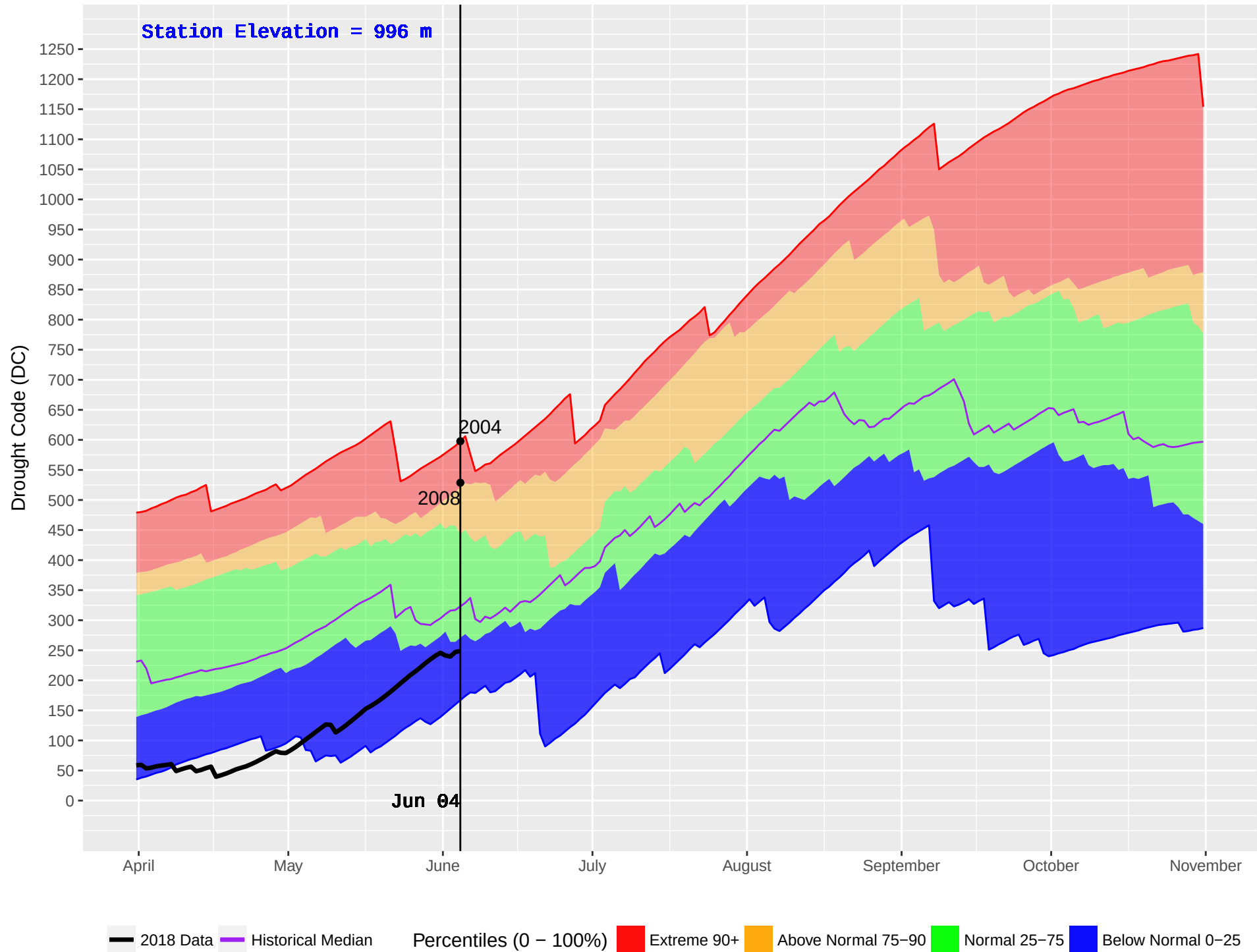
CRANBROOK FS (426) : Historical (2001–2016) and Current (2018) Noon Drought Code (DC)
