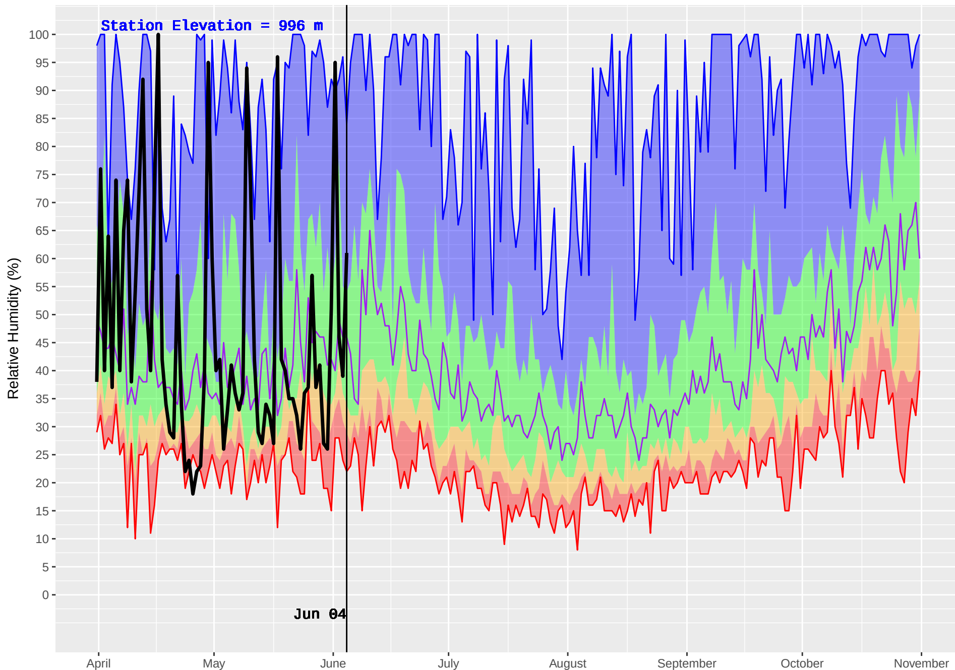
CRANBROOK FS (426) : Historical (2001–2016) and Current (2018) Noon Relative Humidity
