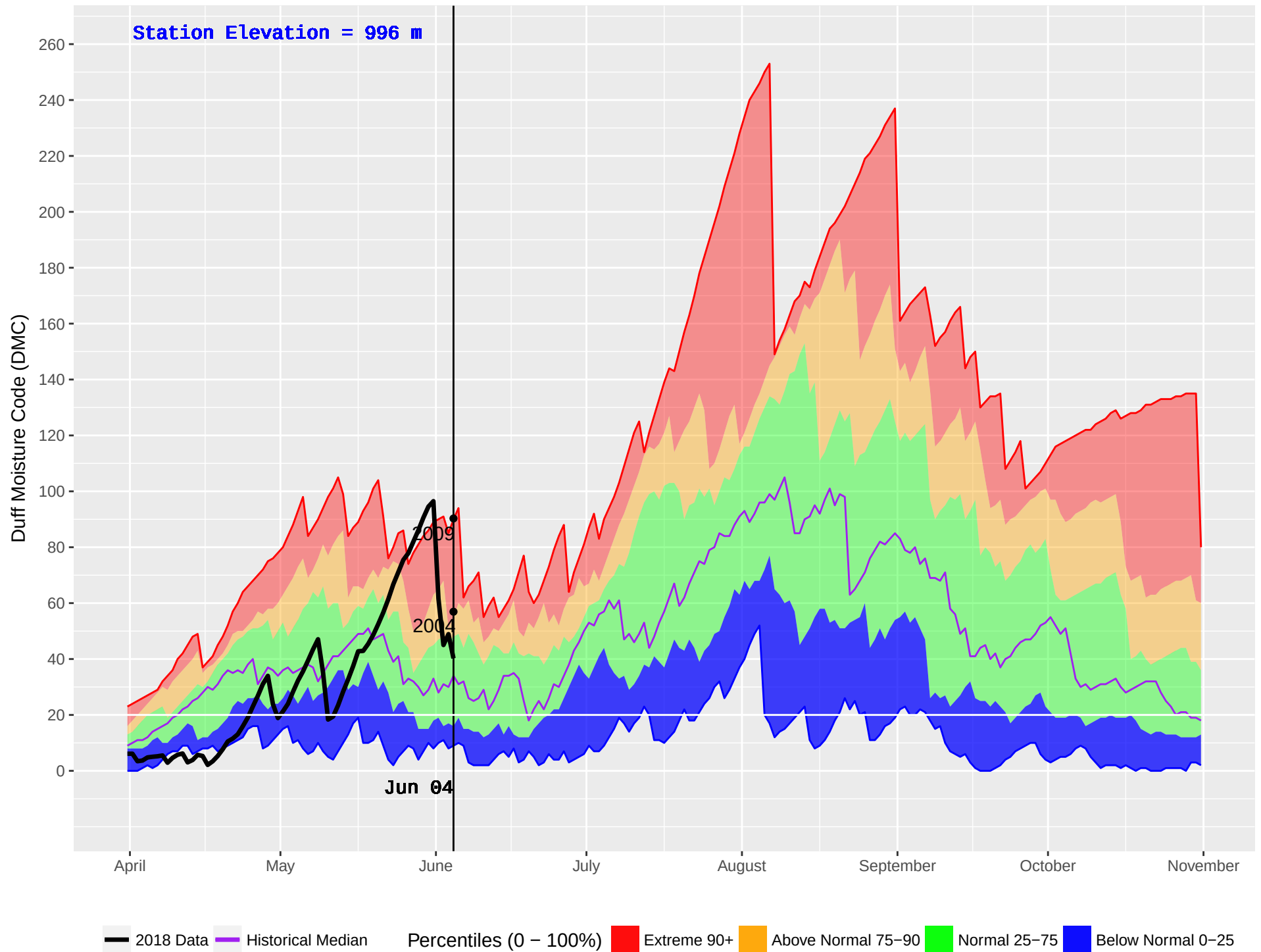
CRANBROOK FS (426) : Historical (2001–2016) and Current (2018) Noon Duff Moisture Code (DMC)
