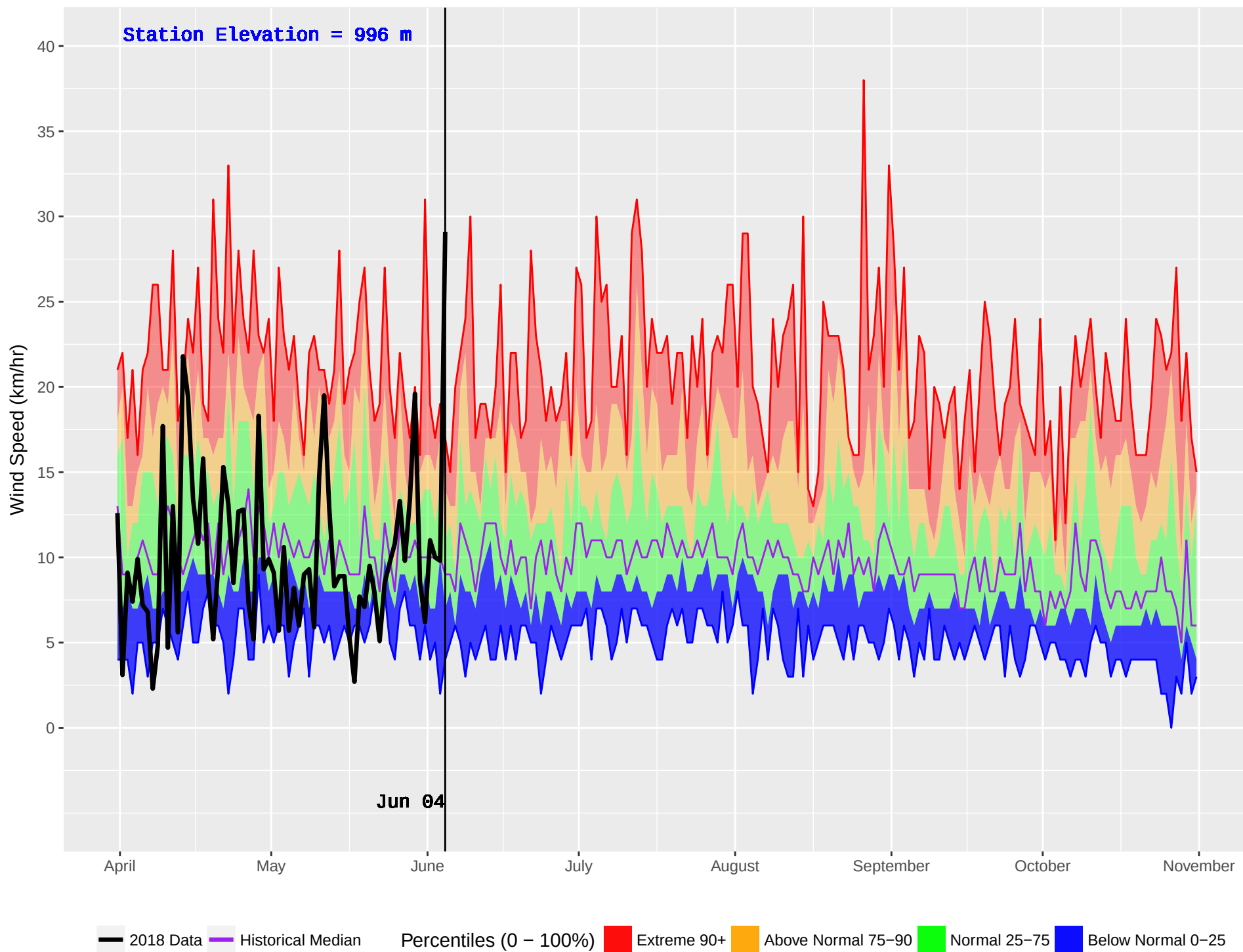
CRANBROOK FS (426) : Historical (2001–2016) and Current (2018) Noon Wind Speed
