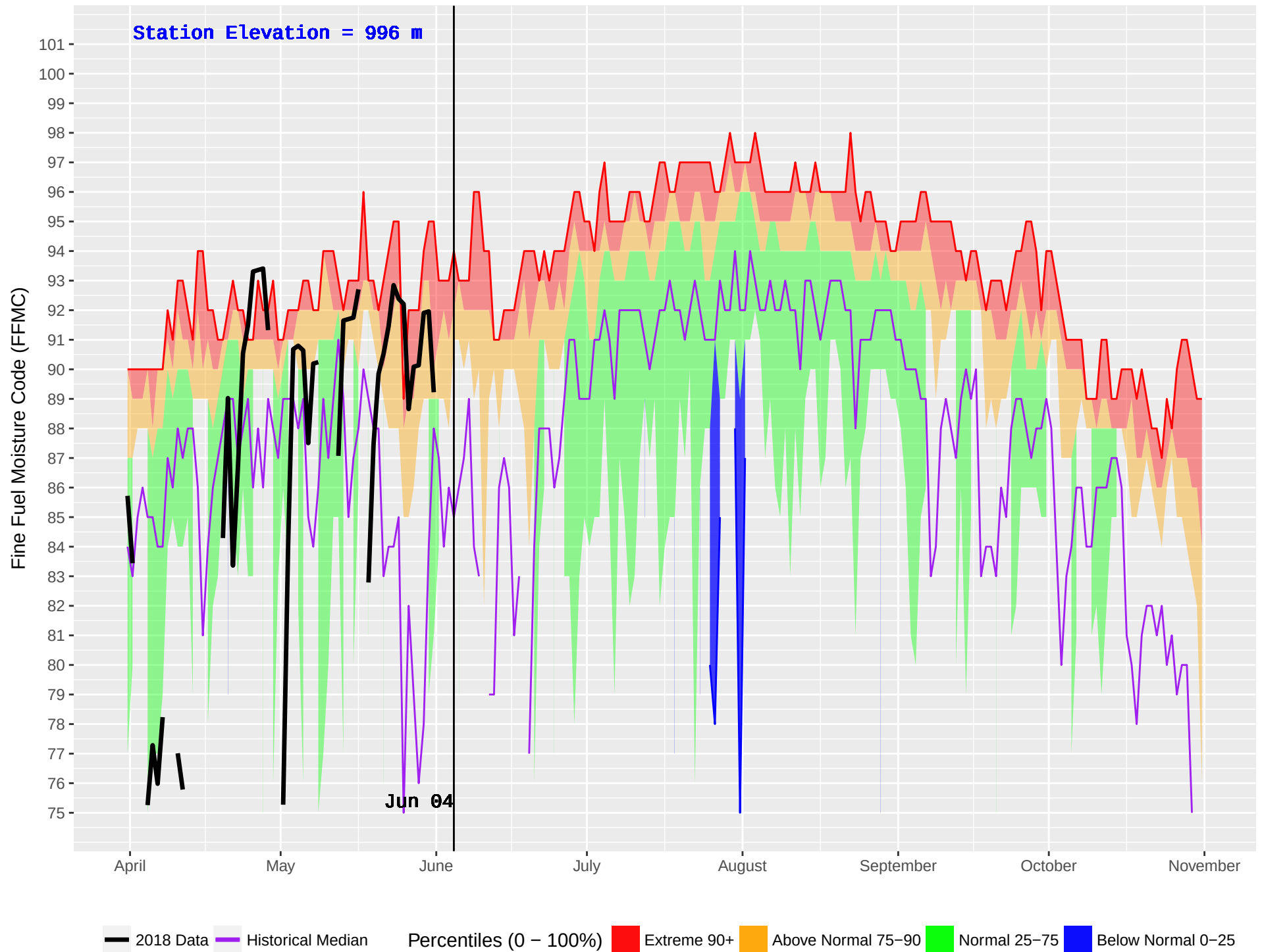
CRANBROOK FS (426) : Historical (2001–2016) and Current (2018) Noon Fine Fuel Moisture Code (FFMC)
