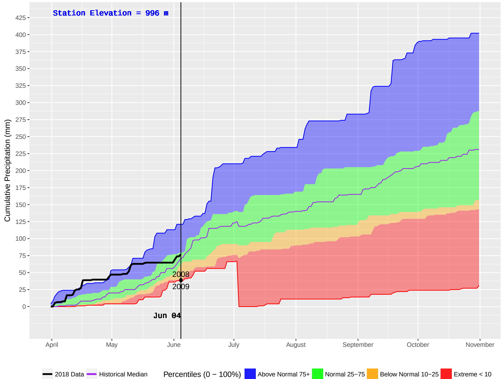
CRANBROOK FS (426) : Historical (2001–2016) and Current (2018) Noon Cumulative Precipitation
