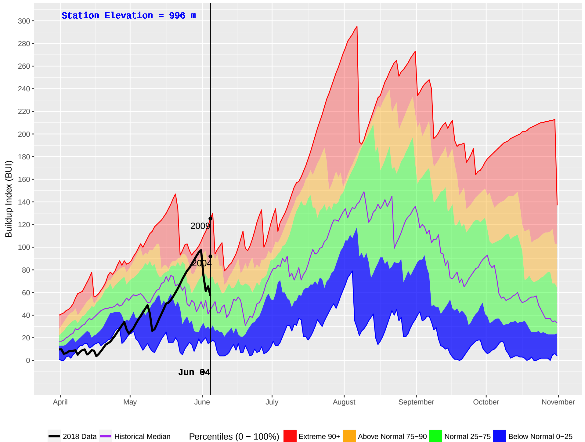
CRANBROOK FS (426) : Historical (2001–2016) and Current (2018) Noon Buildup Index (BUI)
